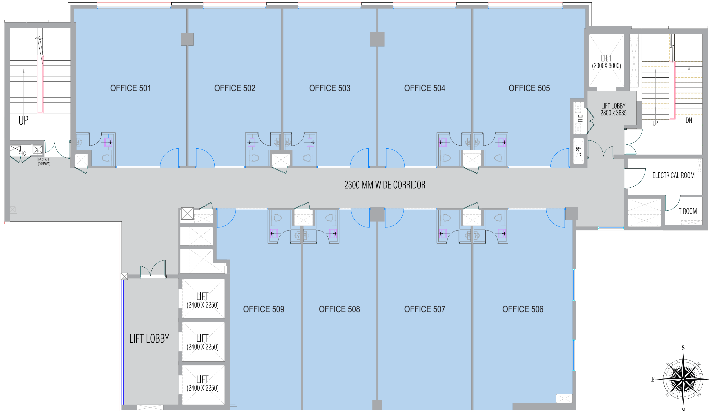
Tower 4A Fifth Floor
