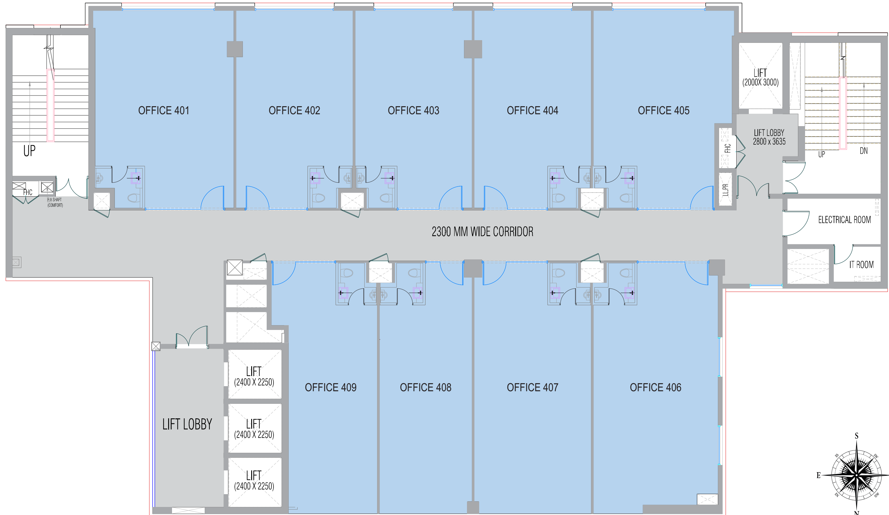
Tower 4A Fourth Floor
