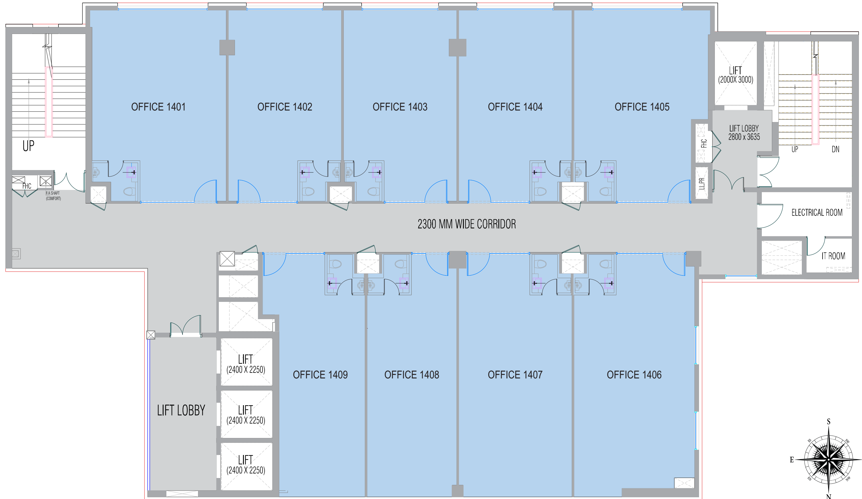
Tower 4A Fourteenth Floor
