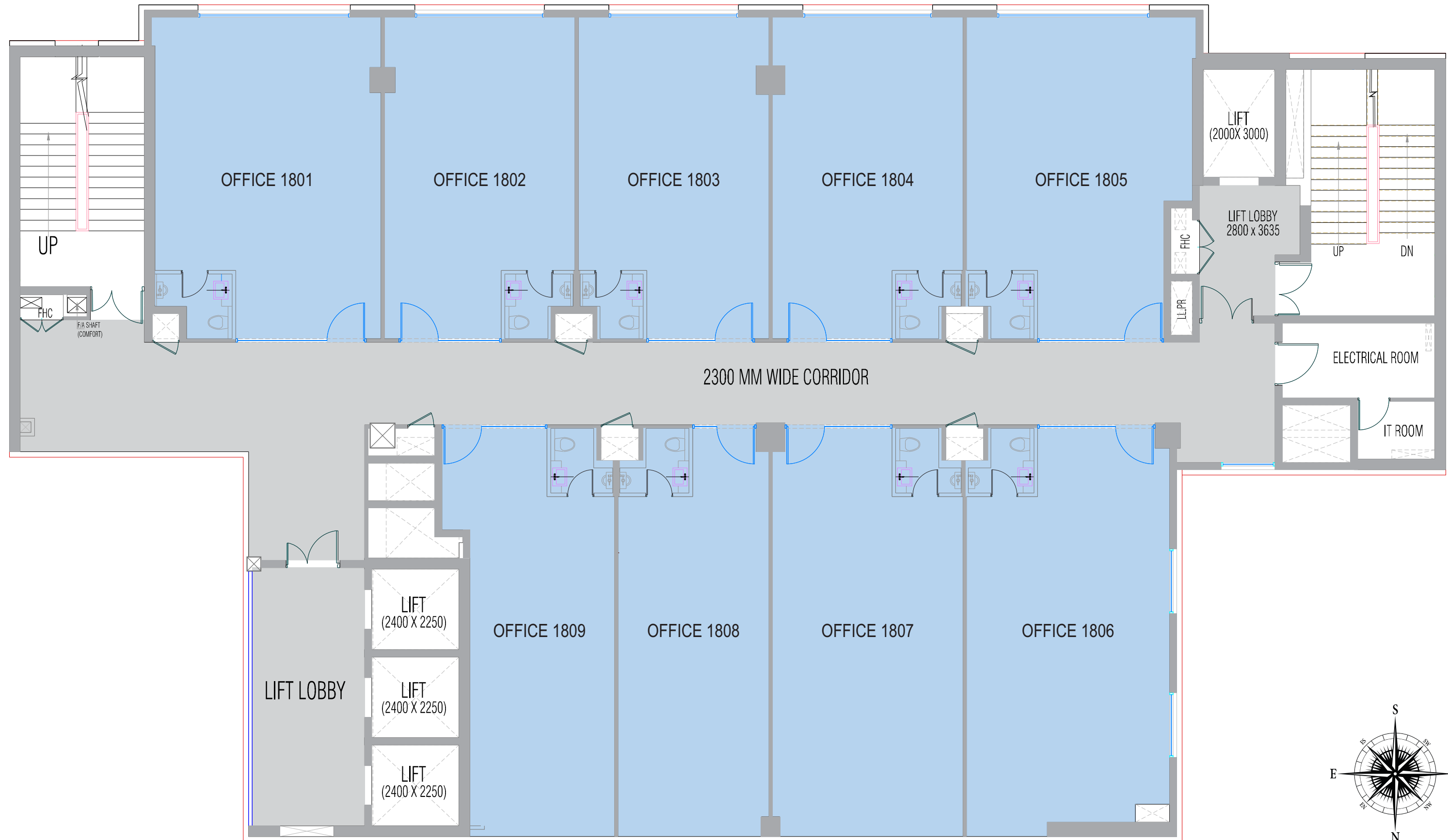
Tower 4A Eighteenth Floor
