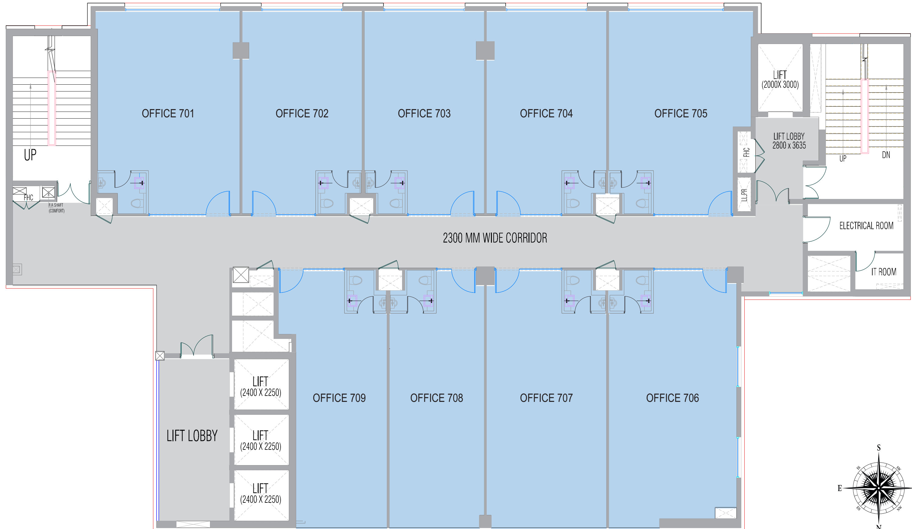
Tower 4A Seventh Floor
