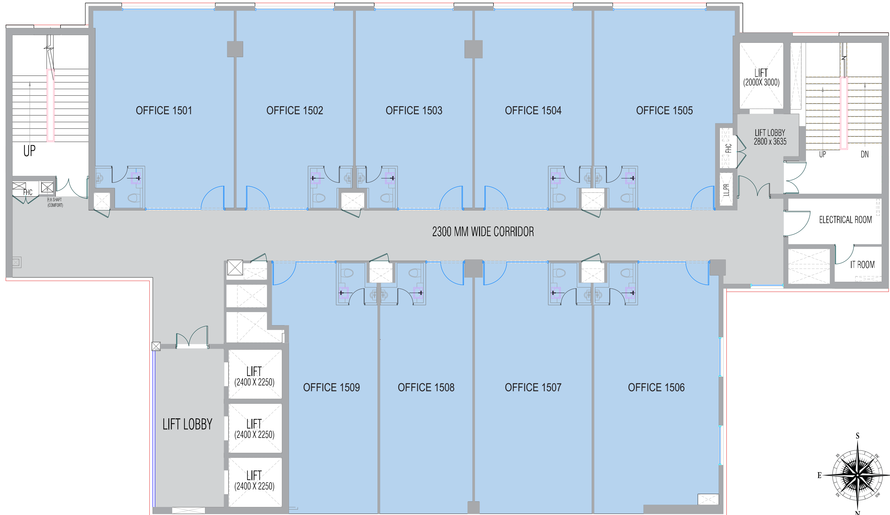
Tower 4A Fifteenth Floor
