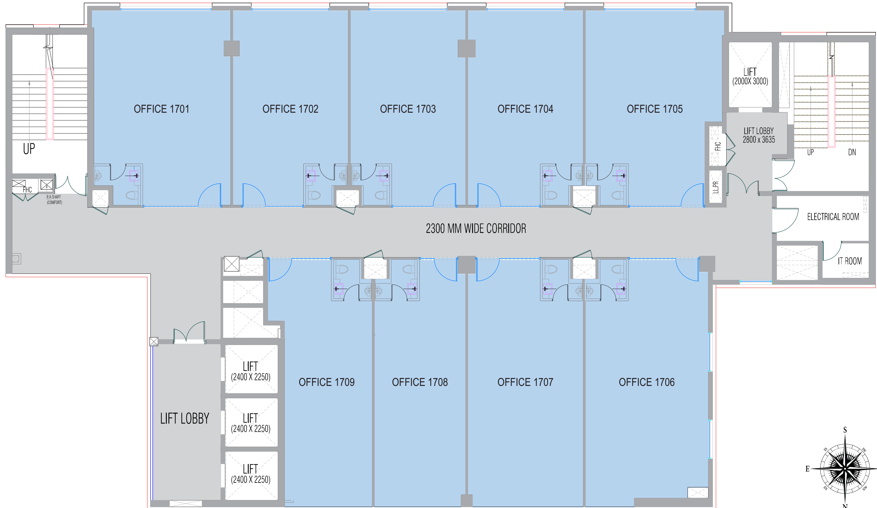
Tower 4A Seventeenth Floor
