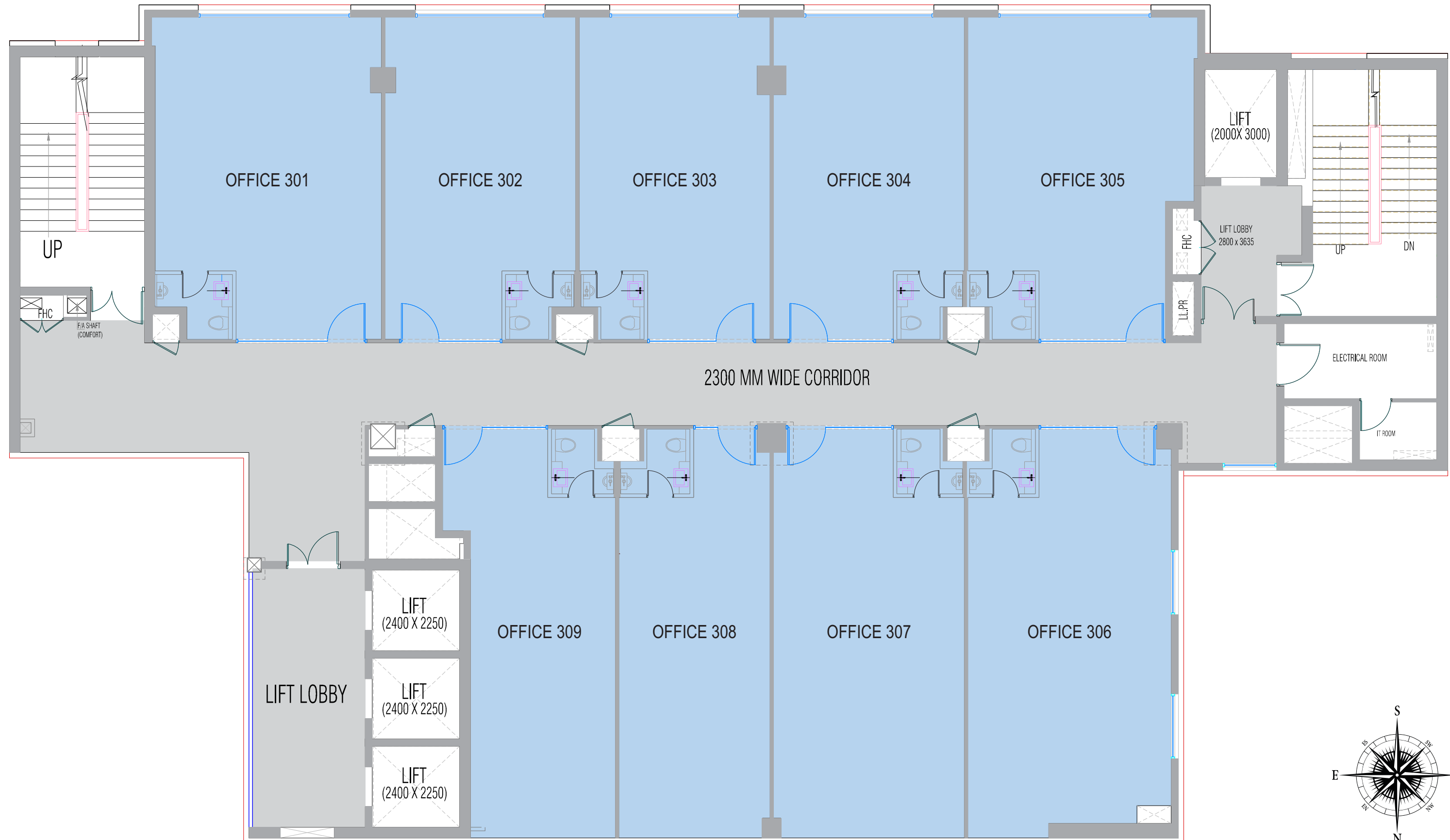
Tower 4A Third Floor
